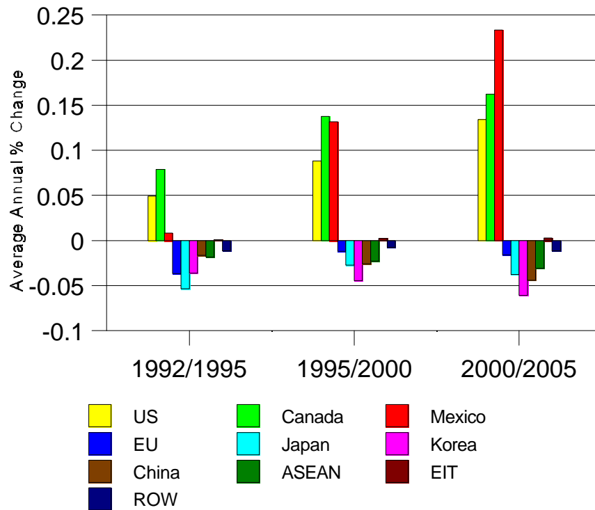
Figure 18 Equivalent Variation
